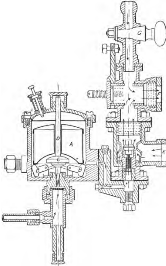
FIG. 318.—The Longuemare Float Feed Carburettor. A is the float; B, B, the weighted levers controlling the needle valve; C, the weight holding the needle valve closed while the lever is right in the float chamber; D, the spindle of the needle valve; E, air inlet; F, pipe communicating to combustion space of cylinder; G, cock for admitting additional air supply.
